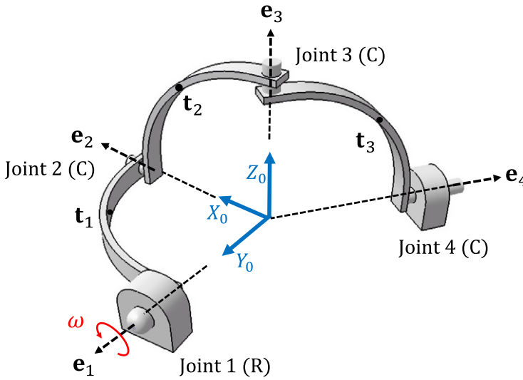
Figure 5. Spherical four-bar linkage.
